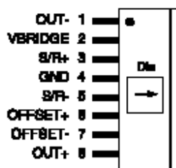
HMC1021Z
