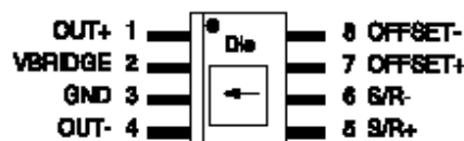
HMC1021S
